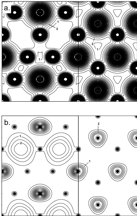
FIG. 6: \beta - \text{Li}_3\text{N} valence density (a) and (unoccupied) inter-layer band density (b) contours perpendicular to the basal plane (left panels) and within the basal plane (right panels). Large regions of white space in (a) signify very low density whereas the contours in the same areas in (b) denote a maximum in the IL density. Contour lines are labeled in units of 0.1 e/\text{\AA}^3 and separated by 0.05 e/\text{\AA}^3 .
