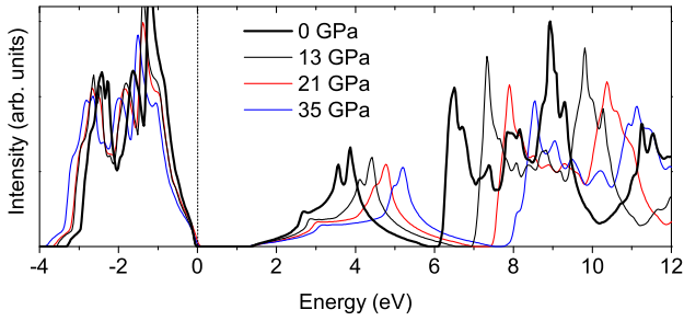
FIG. 7: (Color online) Total density of states of valence and low-lying conduction bands of \beta - \text{Li}_3\text{N} between 0 and 35 GPa.
