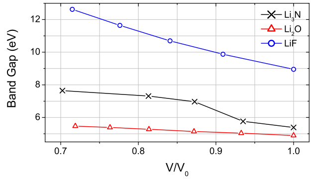
FIG. 10: Band gap increases as a function of volume reduction for related close-shelled cubic Li compounds. \text{LiF} and \text{Li}_2\text{O} are cubic at ambient pressure and V_0 refers to the ambient pressure volume. \text{Li}_3\text{N} V_0 (in this instance alone) is taken as the volume at the \beta \rightarrow \gamma phase transition.
