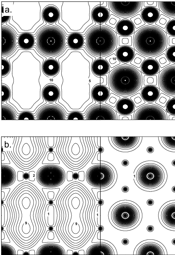
FIG. 5: \alpha - \text{Li}_3\text{N} valence density (a) and (unoccupied) inter-layer band density (b) contours perpendicular to the basal plane (left panels) and within the basal plane (right panels). Large regions of white space in (a) signify very low density whereas the contours in the same areas in (b) denote a maximum in the IL density. Contours are labeled in units of 0.01 e/\text{\AA}^3 and separated by 0.05 e/\text{\AA}^3 (a) and 0.01 e/\text{\AA}^3 (b).
