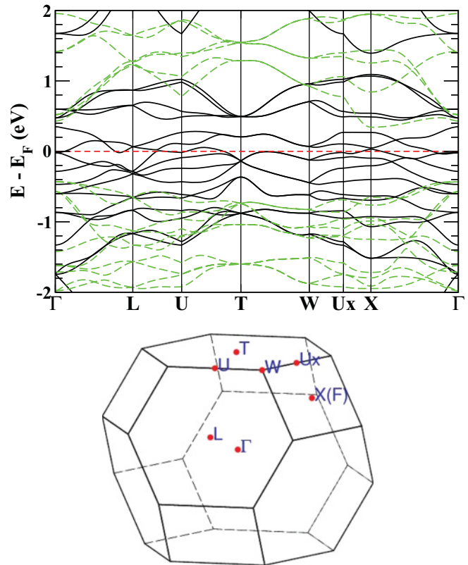
FIG. 2. (Color online) (Top) LSDA band structure near the Fermi energy E_F , where the bands arise only from d orbitals of Ni and Cr ions. The dashed horizontal line indicates E_F , which is taken as the zero of energy. (Bottom) Brillouin zone and high symmetry points of the rhombohedral structure, which has similarity to the fcc Brillouin zone with a threefold axis oriented along the z axis.
