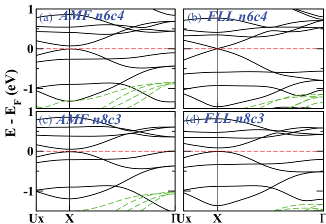
FIG. 4. (Color online) Blowup band structures along the U_x -X- \Gamma line near E_F for various values of U in both schemes of LDA + U. Here, n6c4 denotes U = 6 and 4 eV for Ni and Cr ions, respectively. In panel (b), the gap of 5 meV separates nearly degenerate linear bands similar to what has been observed (at the \Gamma point) in CoSb_3 . 30
