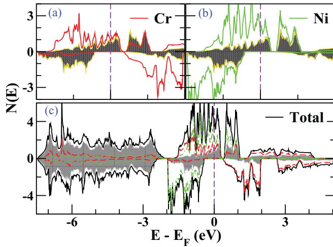
FIG. 3. (Color online) Total and atom-projected LSDA densities of states, which show the half-metallic aspect, expressed per eV-formula unit. In all panels, the shaded regions indicate three oxygen-projected density of states (DOS). The total density of states N(E_F) at E_F is 3.80 states per eV per a formula unit, decomposed of 50% Ni, 30% Cr, and 20% three oxygens characters. (a) Cr 3d DOS in solid line, from -2 to 2 eV; (b) Ni 3d, on same scale as in (a); (c) total DOS in the entire O 2p-metal 3d region. The unoccupied Cr e_g states with the exchange splitting of 1.5 eV lie on 1.5 – 4 eV and 2.5 – 5 eV in the spin-up and spin-down channels, respectively. The exchange splitting of Cr t_{2g} states is about 2 eV. The t_{2g} - e_g crystal field splitting of Cr in the spin-up channel is 3.5 eV, 1 eV larger than in the spin-down channel. The vertical dashed line indicates E_F .
