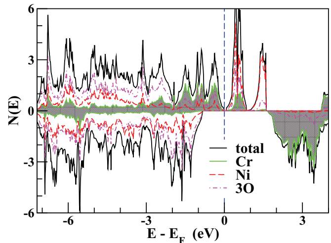
FIG. 5. (Color online) Total and atom-projected densities of states per formula unit in the AMF scheme of LSDA + U using U = 4 and 6 eV for Cr and Ni ions, respectively. Near E_F the occupied part has mostly Cr d character, but the bottom of the unoccupied part has Ni d character even though the strong O characters also exist. In particular, the O characters are nearly the same as the d character in the range of -0.1 – 0.1 eV. This indicates a nearly compensated half-semimetal.
