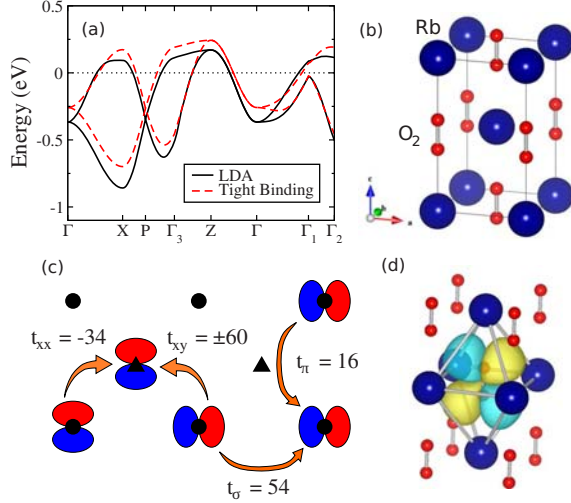
FIG. 1. (Color online) (a) Paramagnetic band plot of \text{RbO}_2 showing bands at the Fermi level from both DFT (LDA) and tight binding. The bands are filled such that there is one hole per site. (b) Conventional unit cell of the tetragonal phase of \text{RbO}_2 . (c) Schematic showing tight-binding hopping parameters in millielectron volt. Circles represent \text{O}_2^- anions in a plane perpendicular to the molecular axis and triangles represent \text{O}_2^- anions in the nearest planes above or below, Rb not shown. (d) Isosurface of the \pi_x^* Wannier function in its local environment. (b) and (d) produced with VESTA (Ref. 19).
